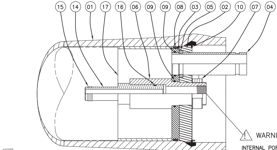
SECTION THROUGH END CLOSURE ITEM 17 DOWNSTREAM ONLY
